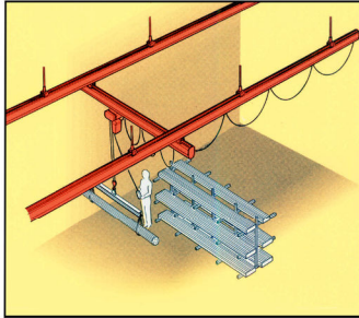
▲ Cross with Single Bridge
