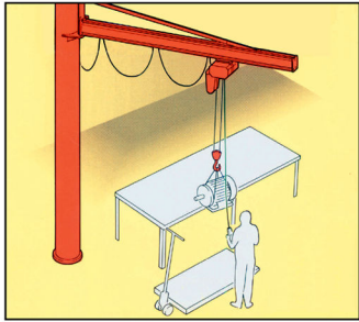
▲ Pillar-mounted Slewing Jib
